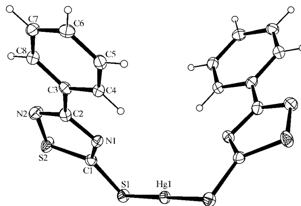
Figure 1 The structure of (I), viewed normal to the twofold axis, showing the atom-numbering scheme. Displacement ellipsoids are drawn at the 50% probability level and H atoms are shown as small spheres of arbitrary radii.
